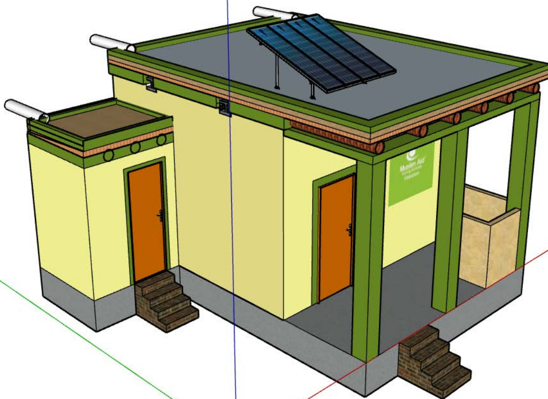
Construction of 50 One room shelter with Toilet and Veranda in District Sanghar Sindh
