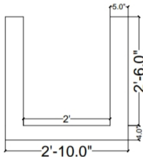
X- Section
