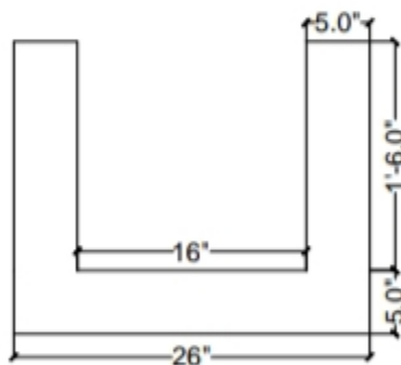
X- Section
