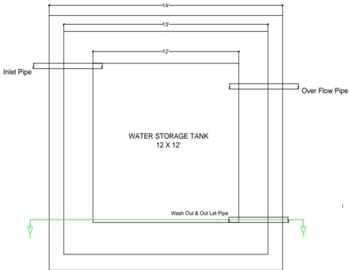
PLAN VIEW D.W.S.S Danine
