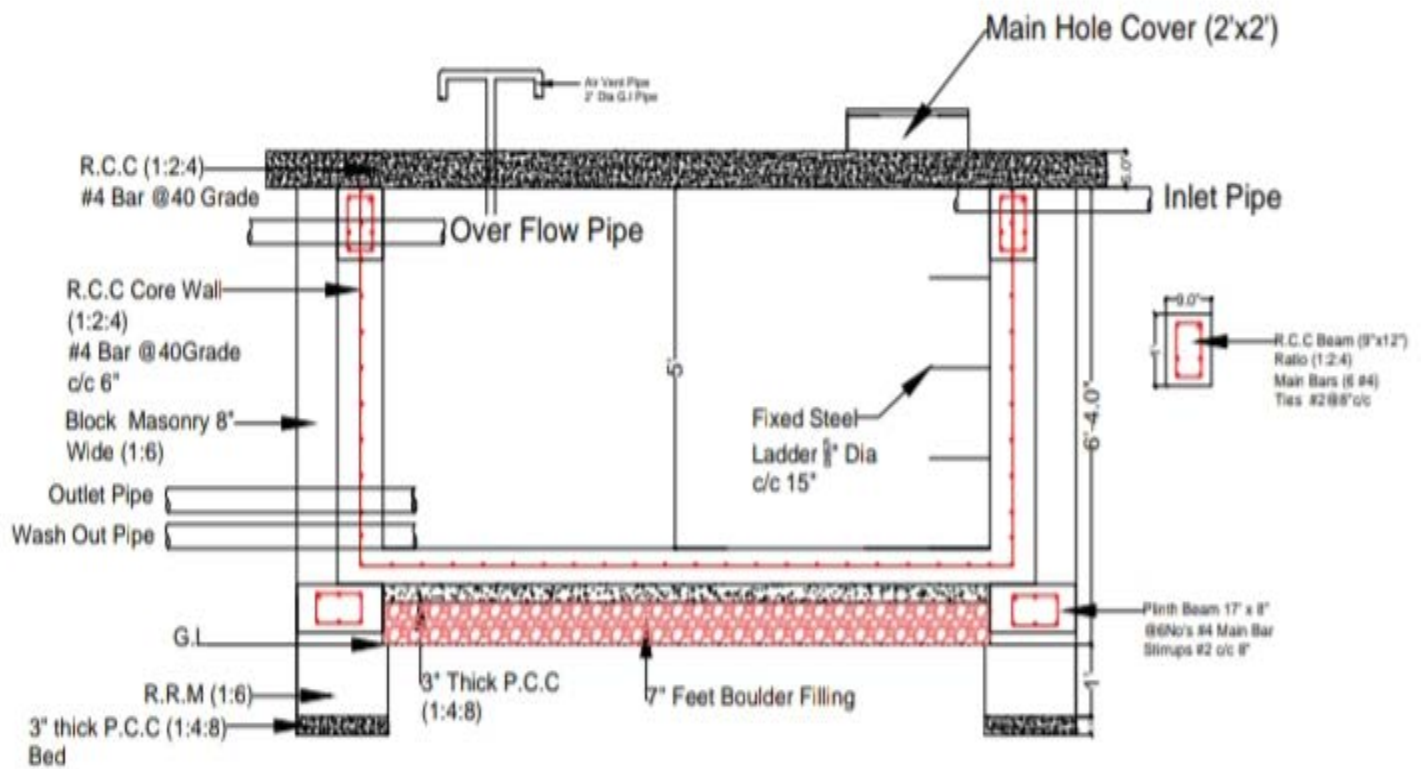
Section of (A-A)
